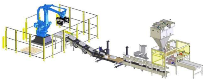
Turnkey Project with bag placer, robot palletizing with MPL165 KG
