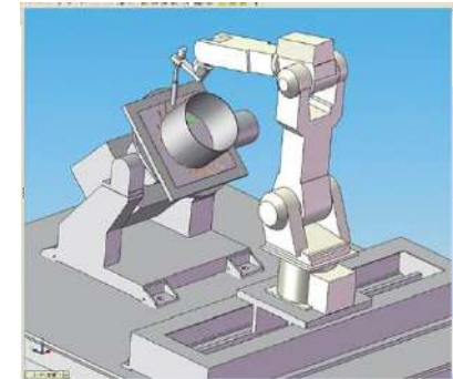
Welding with turning mechanism with MA 1440
